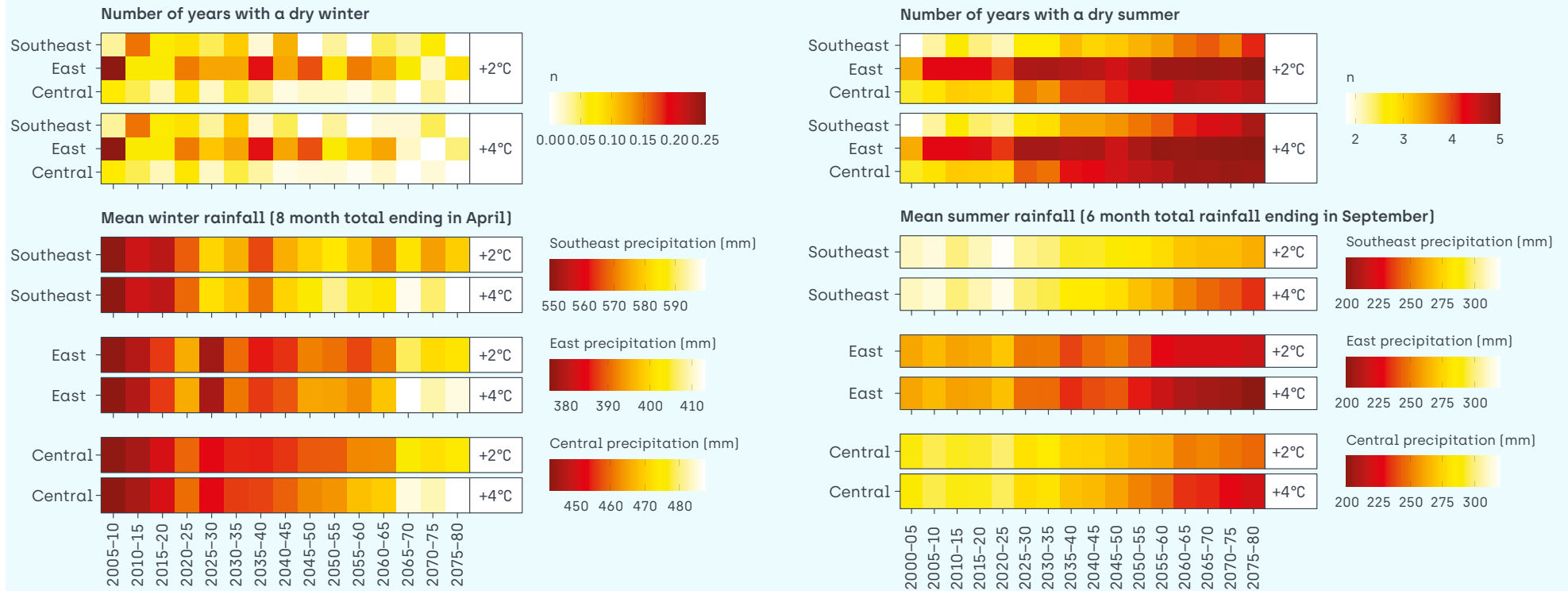
Figure 3-2 - Projections of dry winter and summer precipitation patterns under +2°C and +4°C for our three regions.
