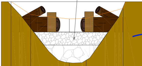
River Cross Section (Large Woody Debris)
